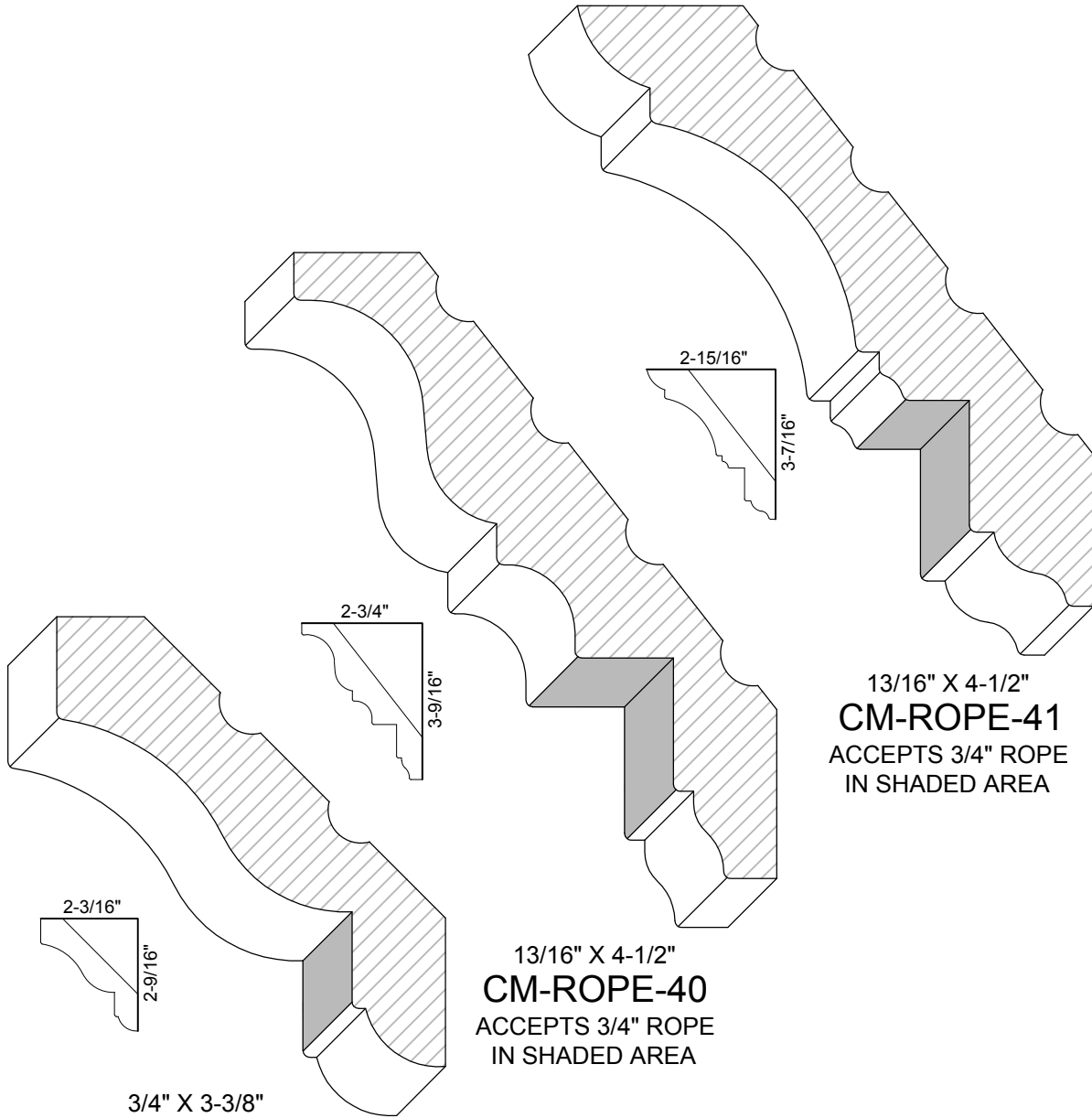
ROPE DETAIL
